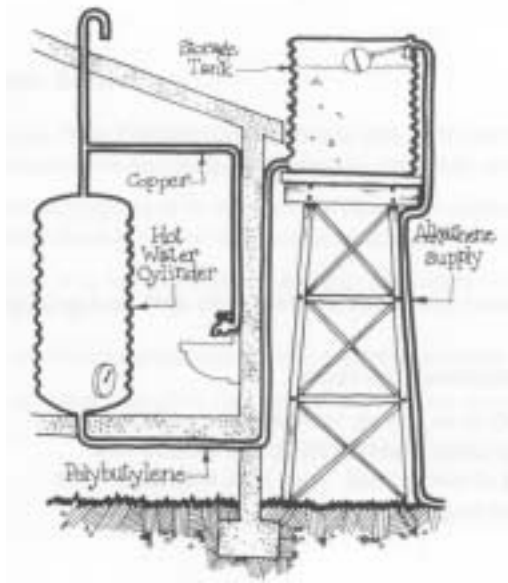
Typical Tank Set Up
