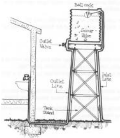
Low cost system
